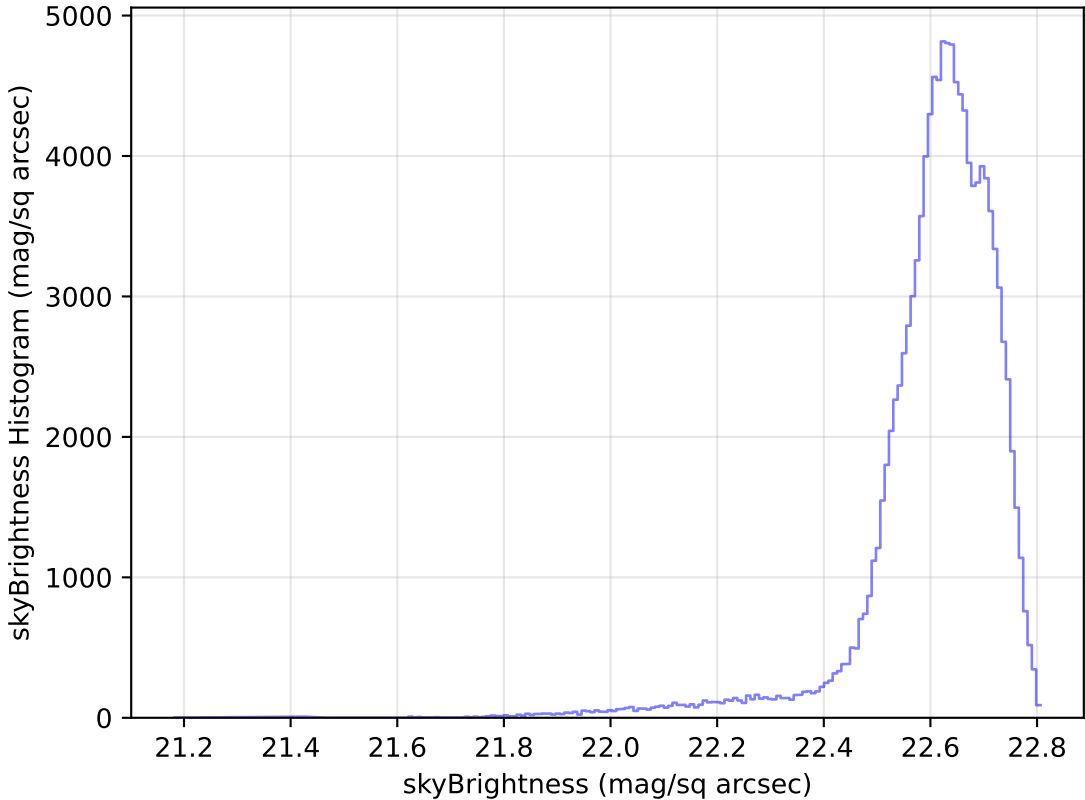
roll_pause_mjdp60_v3.4_10yrs WFD u band: skyBrightness Histogram
