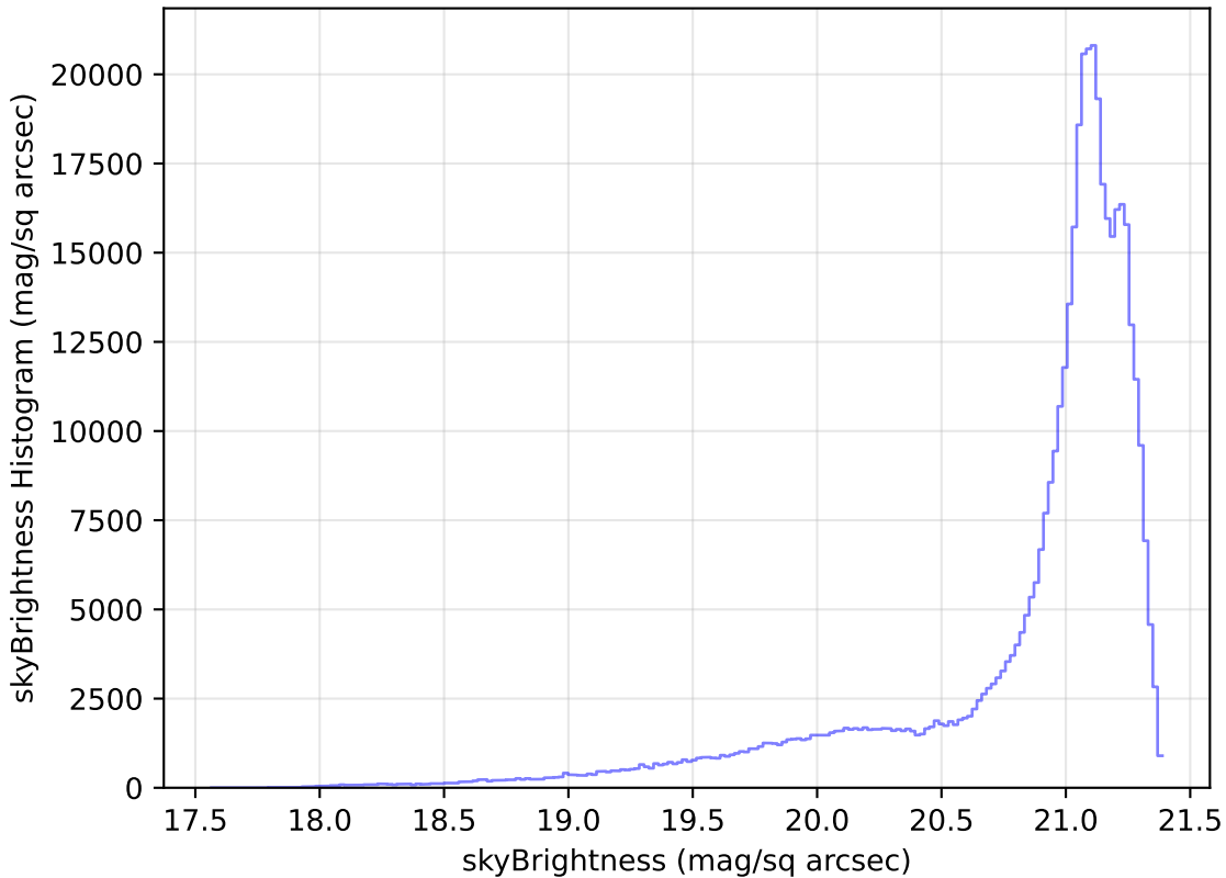
roll_pause_mjdp60_v3.4_10yrs WFD r band: skyBrightness Histogram
