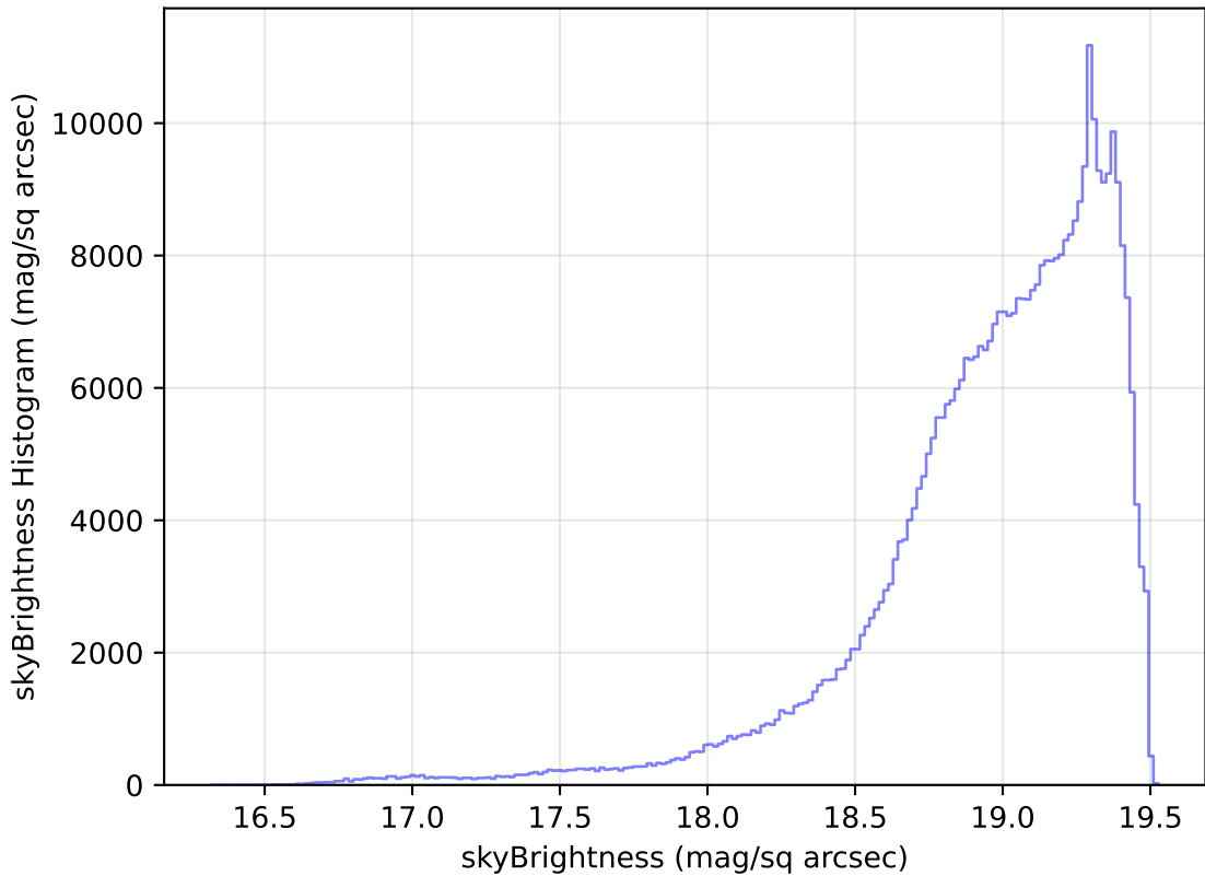
roll_pause_mjdp60_v3.4_10yrs All sky z band: skyBrightness Histogram
