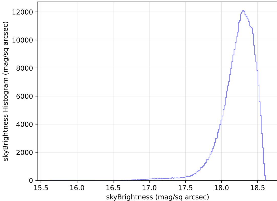
roll_pause_mjdp60_v3.4_10yrs All sky y band: skyBrightness Histogram
