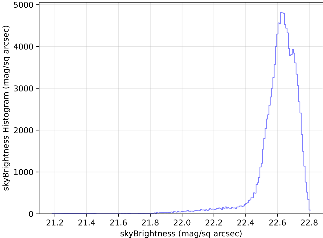
roll_pause_mjdp60_v3.4_10yrs All sky u band: skyBrightness Histogram
