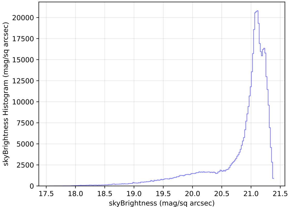
roll_pause_mjdp60_v3.4_10yrs All sky r band: skyBrightness Histogram
