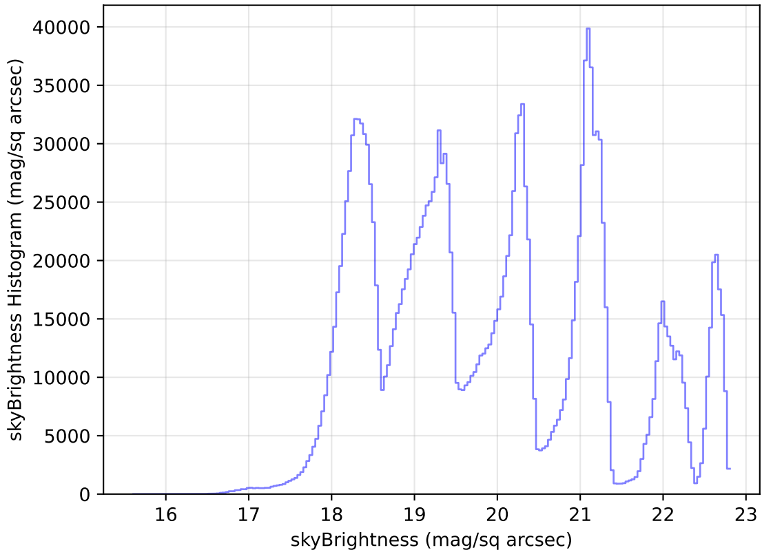
roll_pause_mjdp60_v3.4_10yrs All sky all bands: skyBrightness Histogram
