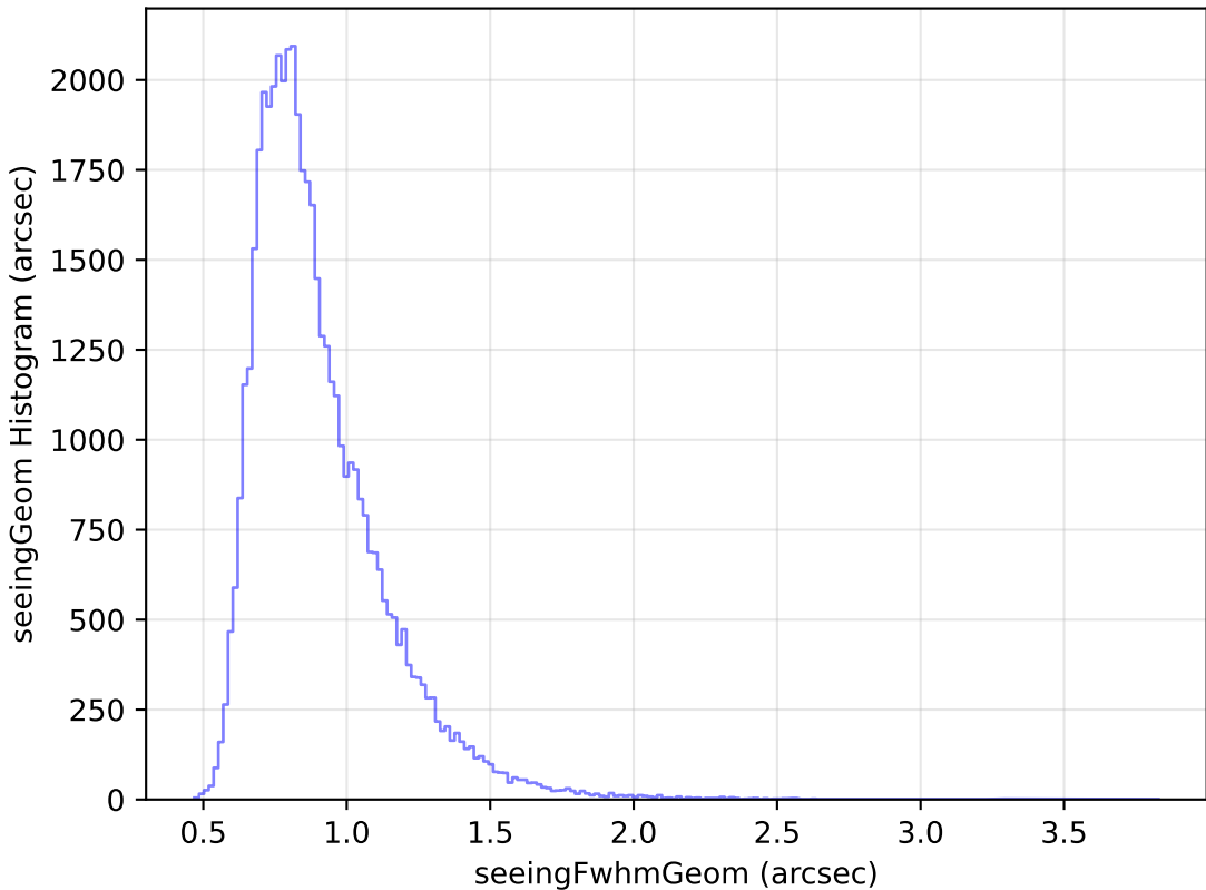
roll_pause_mjdp60_v3.4_10yrs Yr 1 y band: seeingGeom Histogram
