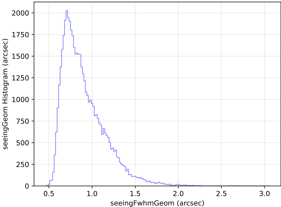
roll_pause_mjdp60_v3.4_10yrs Yr 1 r band: seeingGeom Histogram
