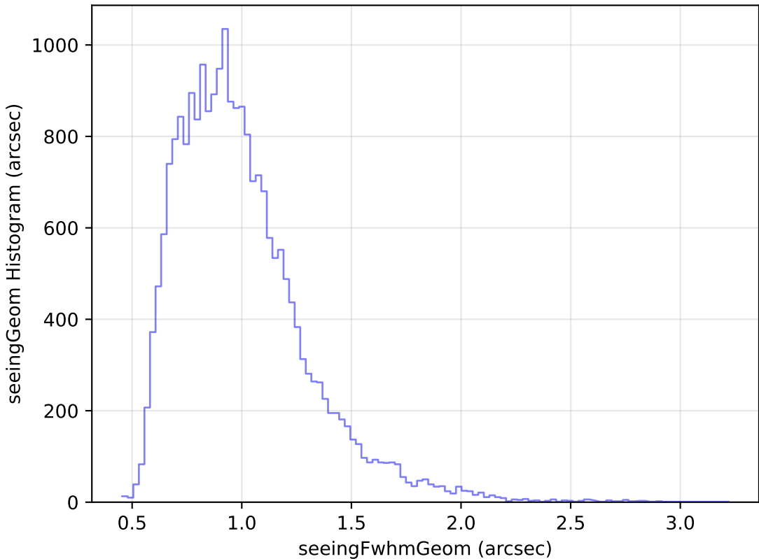
roll_pause_mjdp60_v3.4_10yrs Yr 1 g band: seeingGeom Histogram
