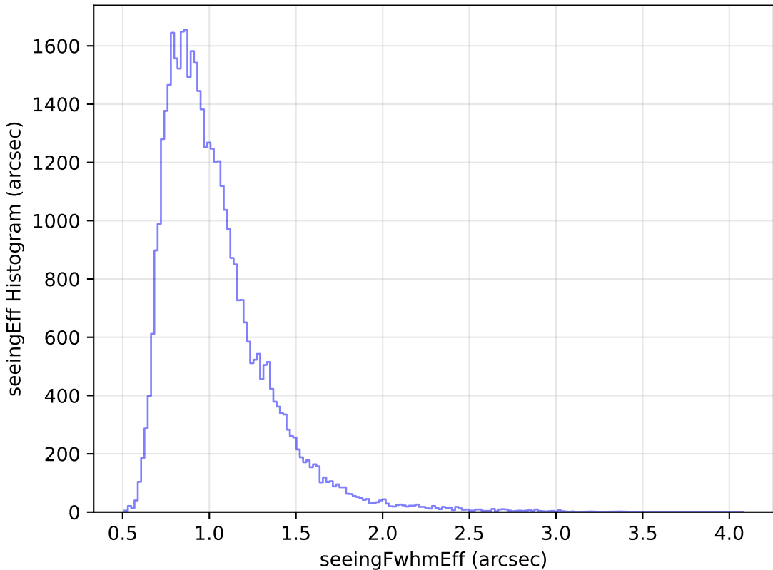
roll_pause_mjdp60_v3.4_10yrs Yr 1 z band: seeingEff Histogram
