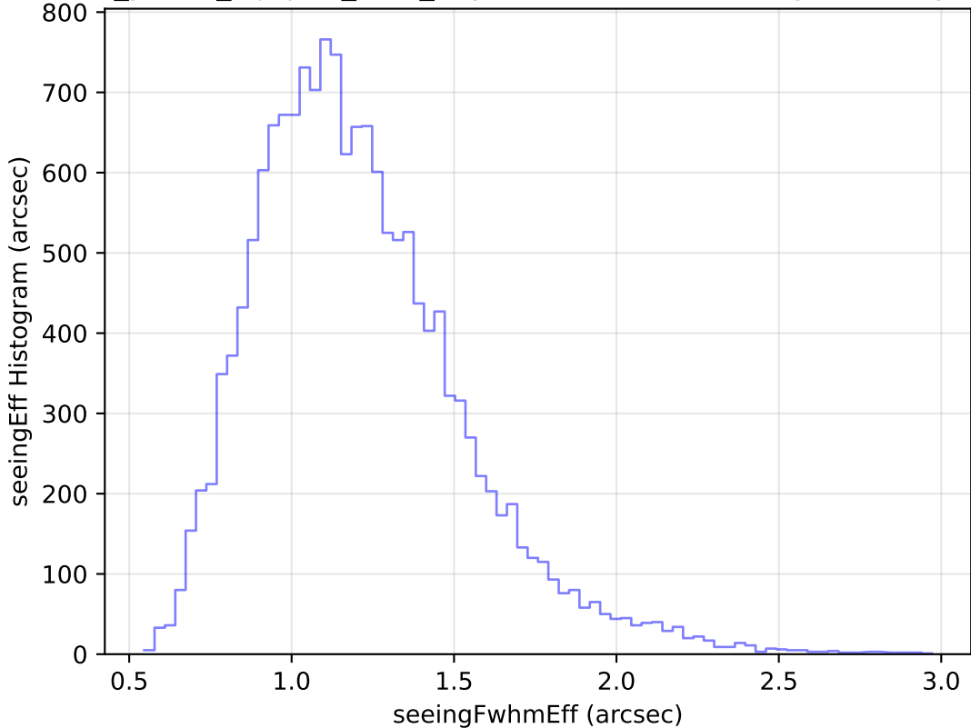
roll_pause_mjdp60_v3.4_10yrs Yr 1 u band: seeingEff Histogram
