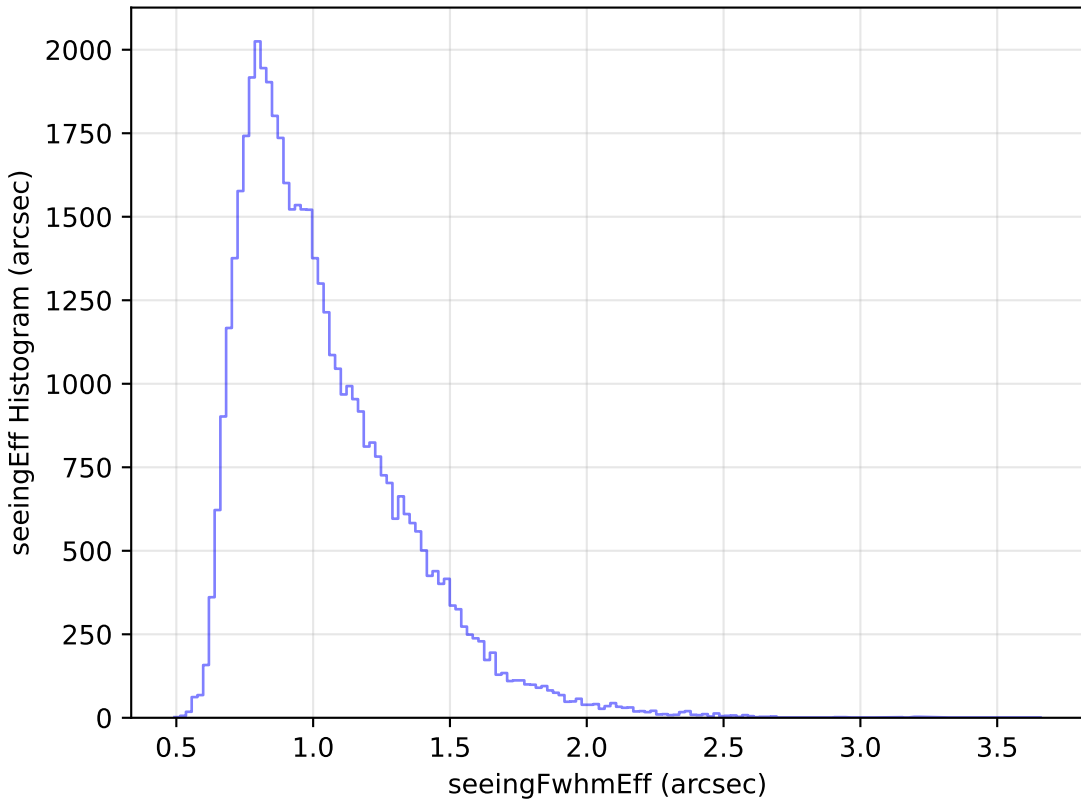
roll_pause_mjdp60_v3.4_10yrs Yr 1 r band: seeingEff Histogram
