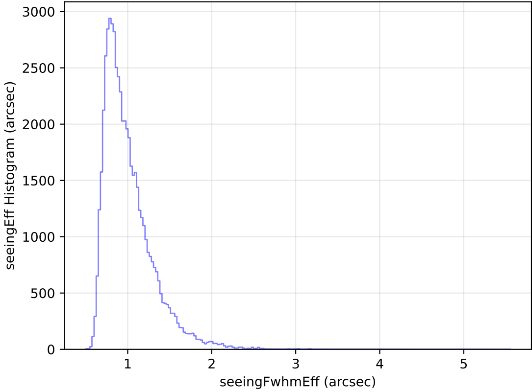
roll_pause_mjdp60_v3.4_10yrs Yr 1 i band: seeingEff Histogram
