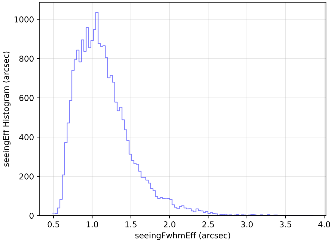
roll_pause_mjdp60_v3.4_10yrs Yr 1 g band: seeingEff Histogram
