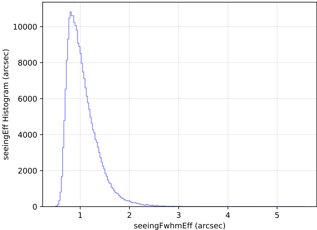
roll_pause_mjdp60_v3.4_10yrs Yr 1 all bands: seeingEff Histogram
