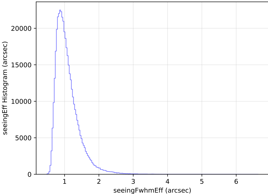
roll_pause_mjdp60_v3.4_10yrs WFD z band: seeingEff Histogram
