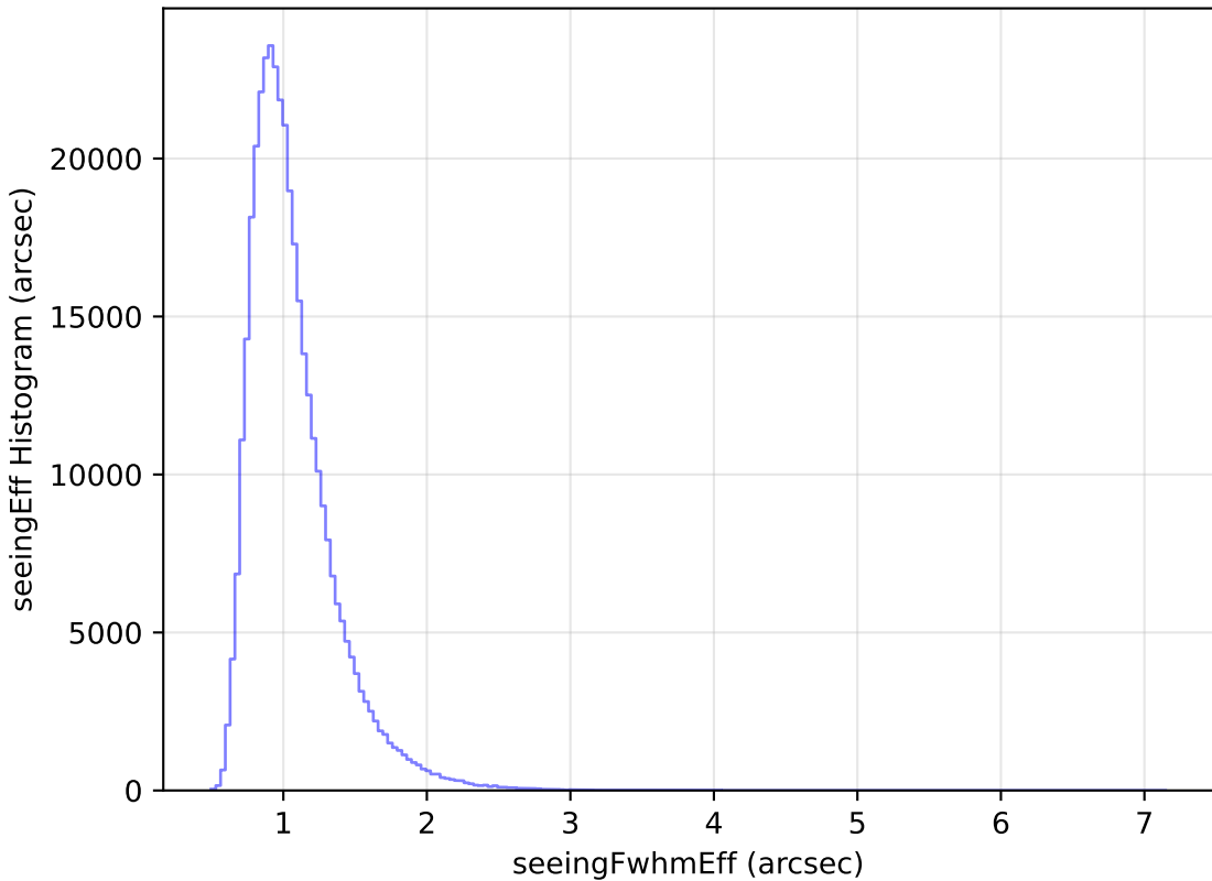
roll_pause_mjdp60_v3.4_10yrs WFD y band: seeingEff Histogram
