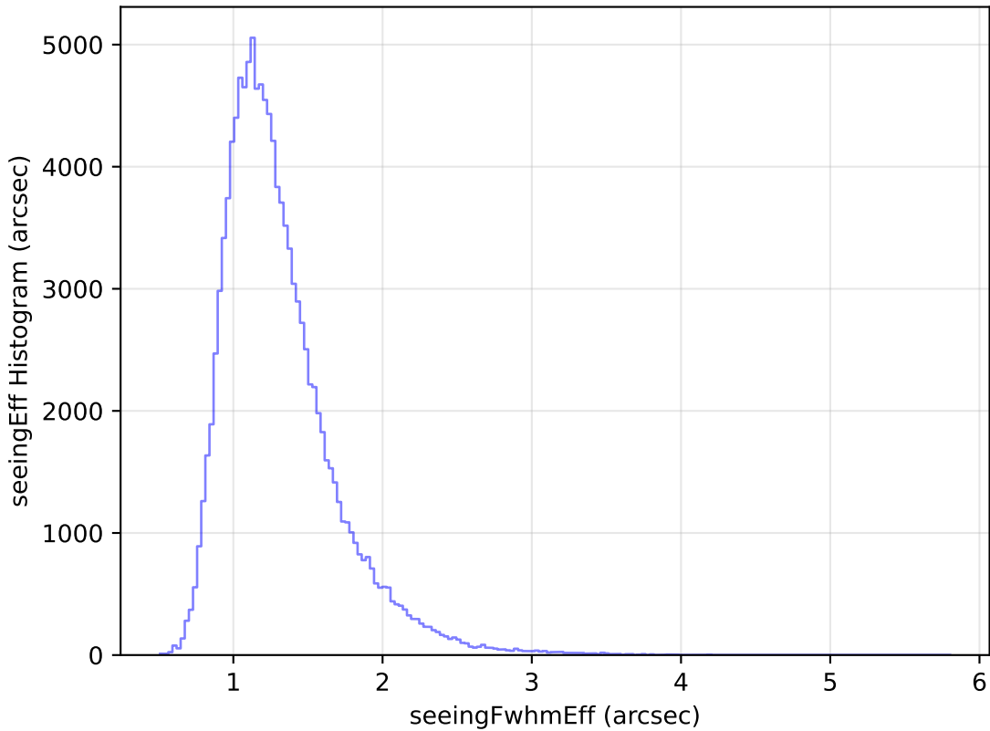
roll_pause_mjdp60_v3.4_10yrs WFD u band: seeingEff Histogram
