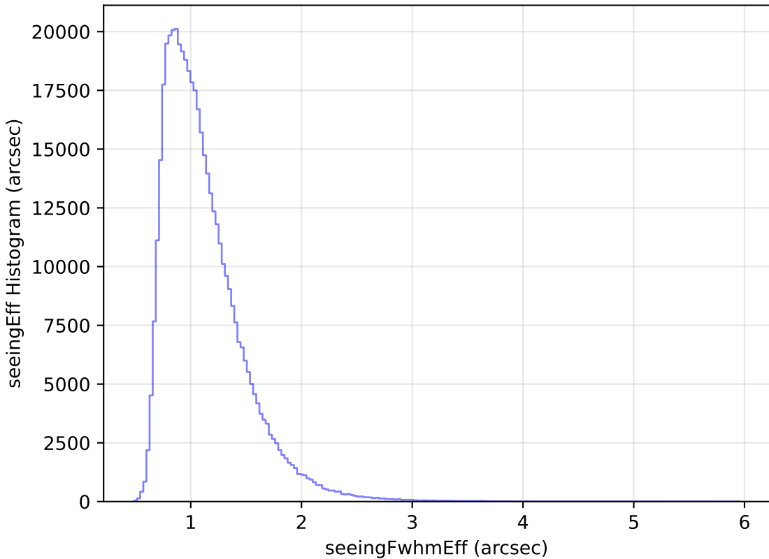
roll_pause_mjdp60_v3.4_10yrs WFD r band: seeingEff Histogram
