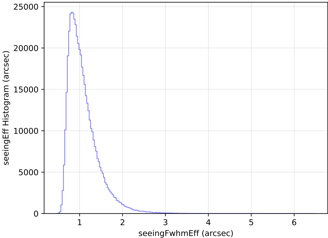
roll_pause_mjdp60_v3.4_10yrs WFD i band: seeingEff Histogram
