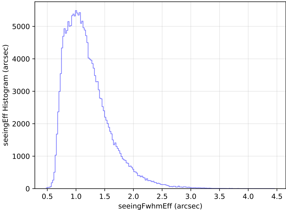
roll_pause_mjdp60_v3.4_10yrs WFD g band: seeingEff Histogram
