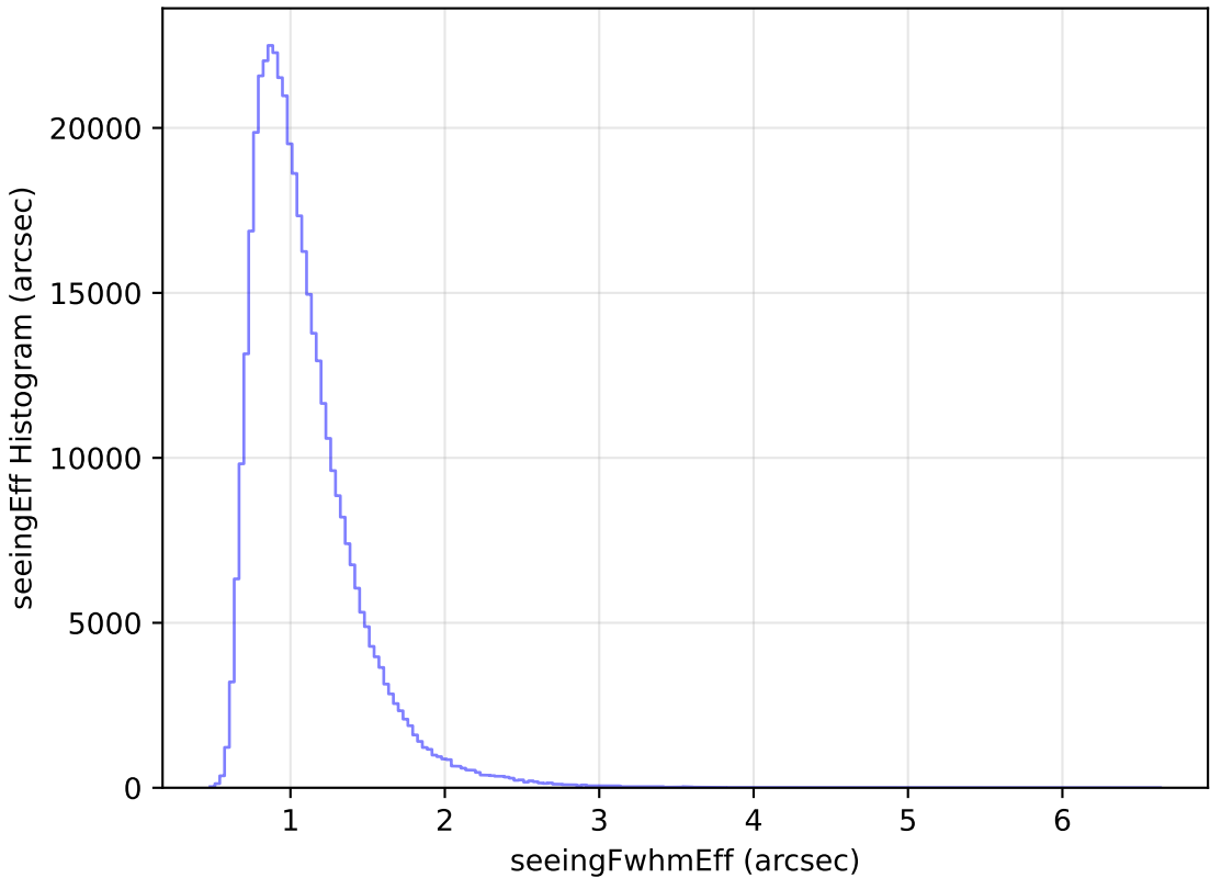
roll_pause_mjdp60_v3.4_10yrs All sky z band: seeingEff Histogram
