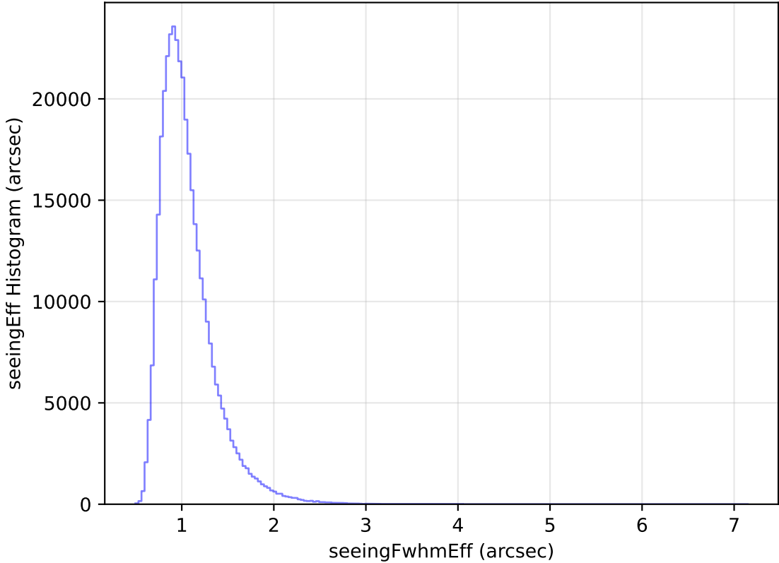
roll_pause_mjdp60_v3.4_10yrs All sky y band: seeingEff Histogram
