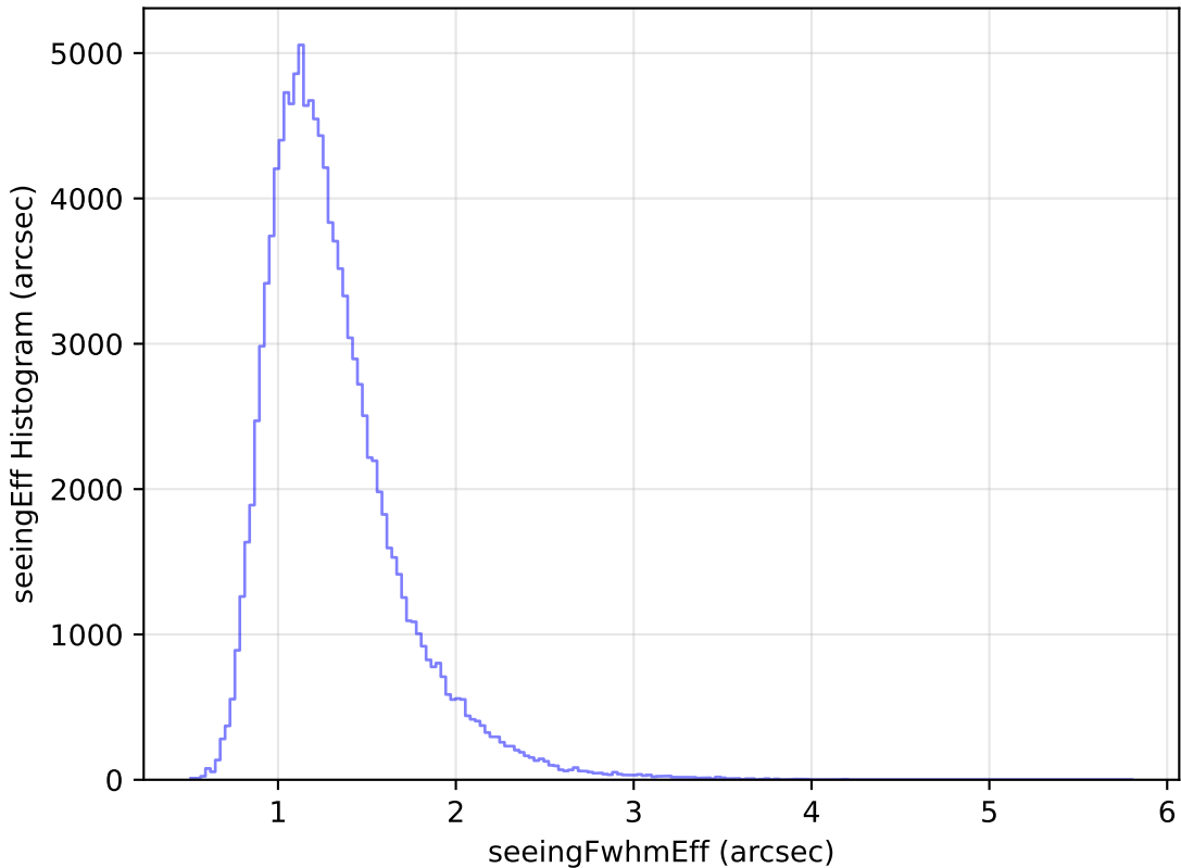
roll_pause_mjdp60_v3.4_10yrs All sky u band: seeingEff Histogram
