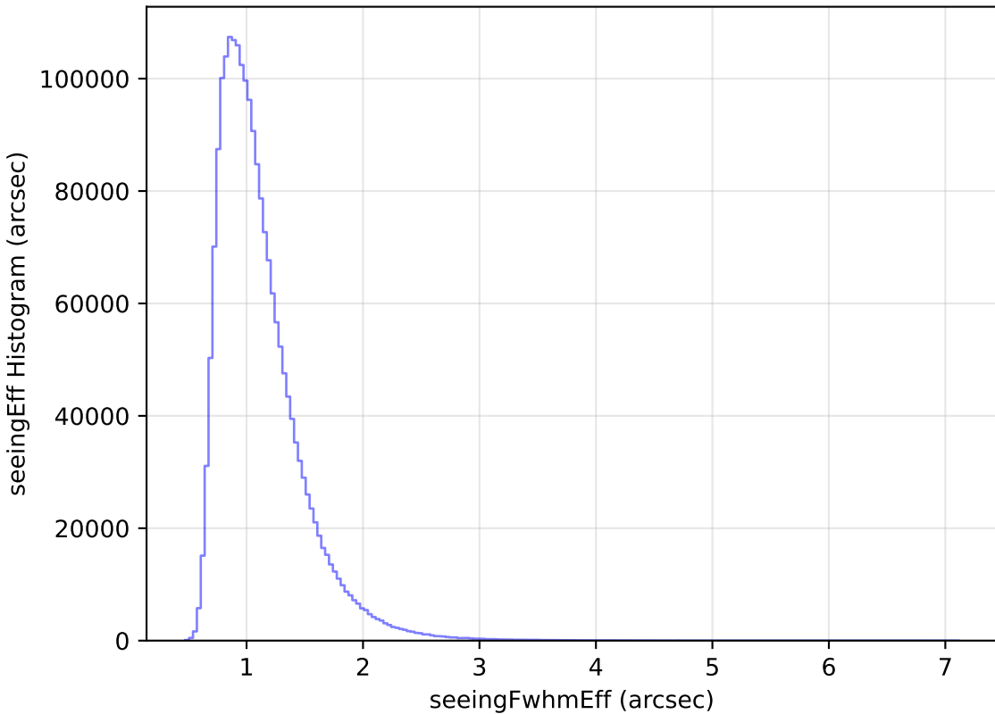
roll_pause_mjdp60_v3.4_10yrs All sky all bands: seeingEff Histogram
