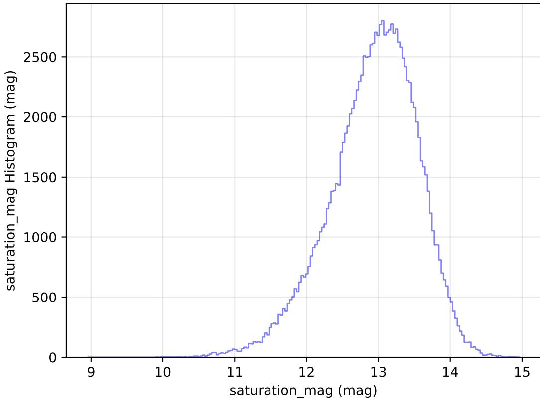
roll_pause_mjdp60_v3.4_10yrs WFD u band: saturation_mag Histogram
