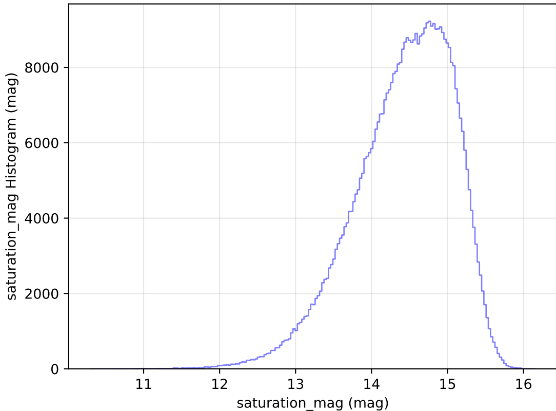
roll_pause_mjdp60_v3.4_10yrs WFD i band: saturation_mag Histogram
