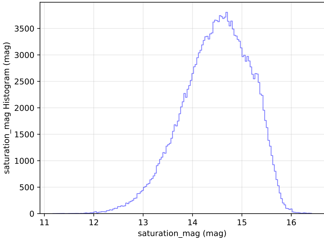
roll_pause_mjdp60_v3.4_10yrs WFD g band: saturation_mag Histogram
