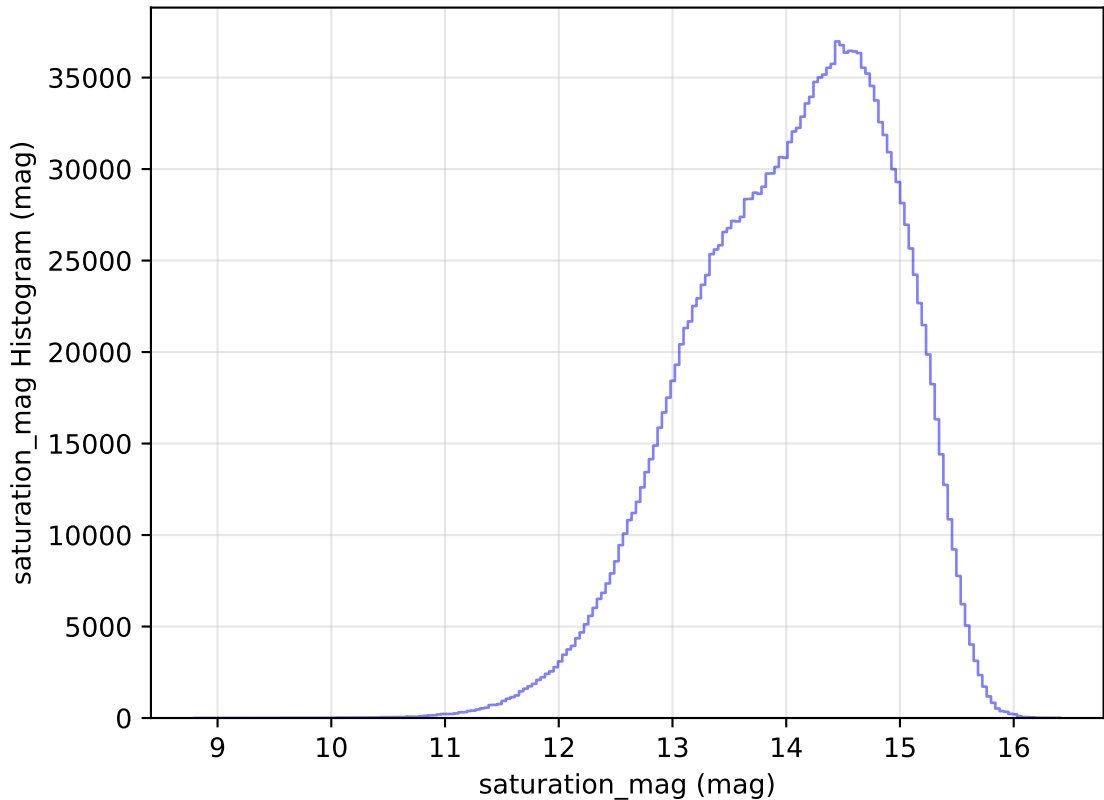
roll_pause_mjdp60_v3.4_10yrs WFD all bands: saturation_mag Histogram
