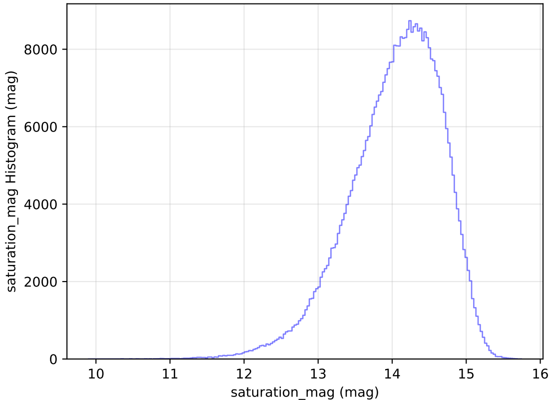
roll_pause_mjdp60_v3.4_10yrs All sky z band: saturation_mag Histogram
