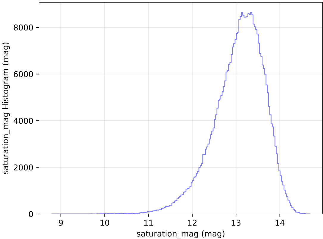
roll_pause_mjdp60_v3.4_10yrs All sky y band: saturation_mag Histogram
