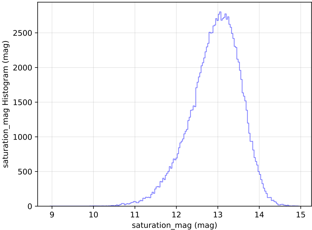
roll_pause_mjdp60_v3.4_10yrs All sky u band: saturation_mag Histogram
