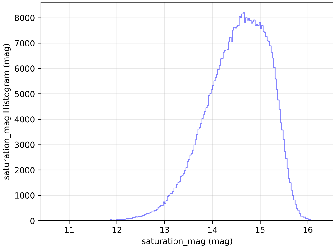
roll_pause_mjdp60_v3.4_10yrs All sky r band: saturation_mag Histogram
