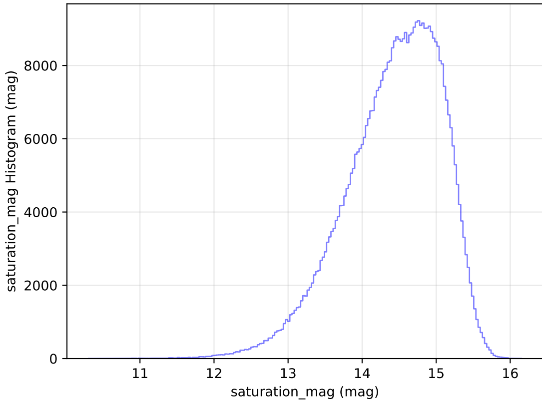
roll_pause_mjdp60_v3.4_10yrs All sky i band: saturation_mag Histogram
