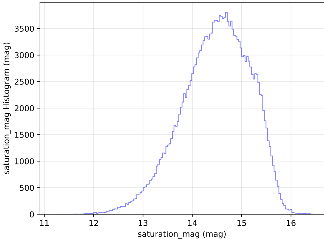
roll_pause_mjdp60_v3.4_10yrs All sky g band: saturation_mag Histogram
