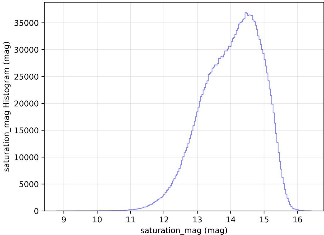
roll_pause_mjdp60_v3.4_10yrs All sky all bands: saturation_mag Histogram
