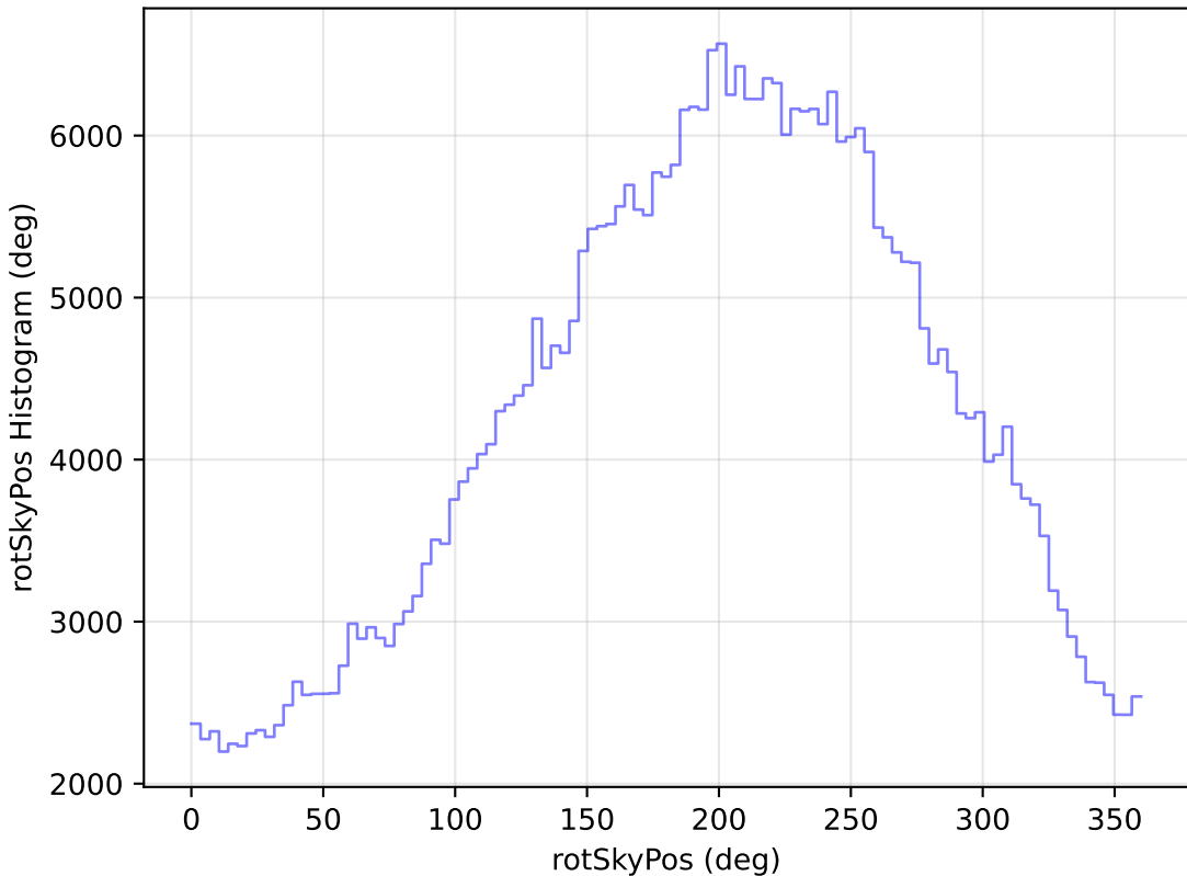
roll_pause_mjdp60_v3.4_10yrs WFD z band: rotSkyPos Histogram
