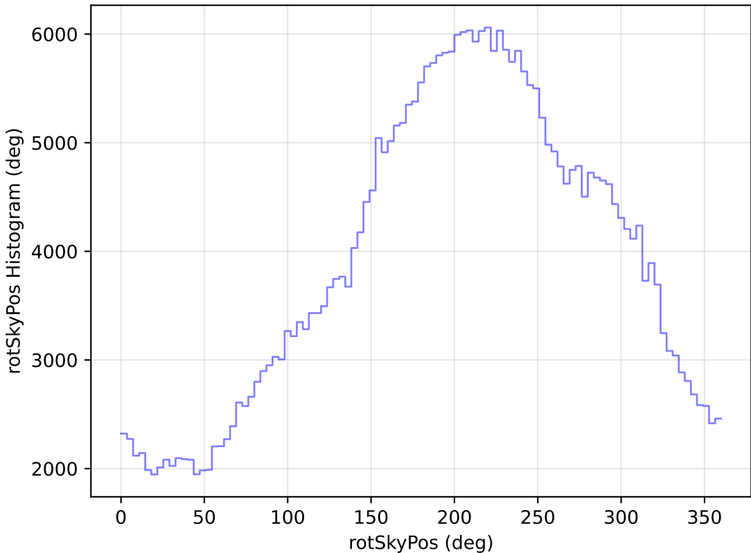
roll_pause_mjdp60_v3.4_10yrs WFD y band: rotSkyPos Histogram
