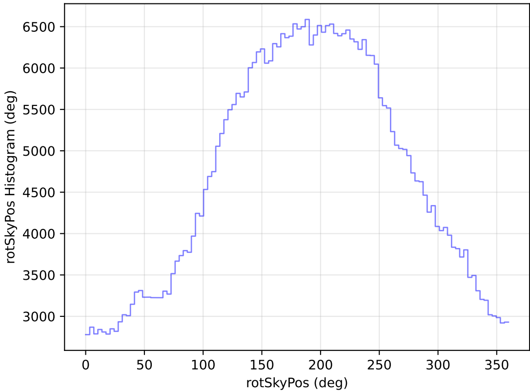
roll_pause_mjdp60_v3.4_10yrs WFD r band: rotSkyPos Histogram
