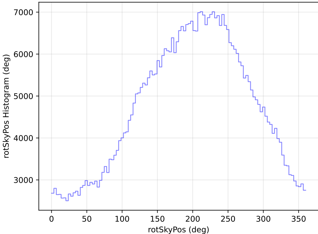
roll_pause_mjdp60_v3.4_10yrs WFD i band: rotSkyPos Histogram
