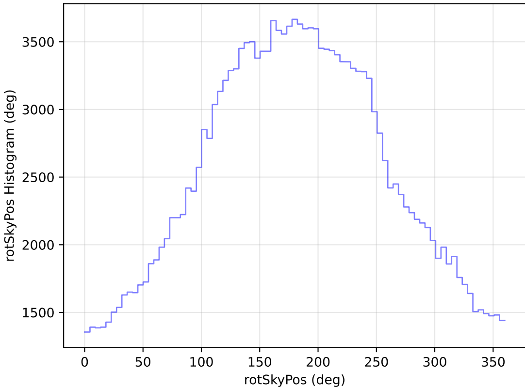
roll_pause_mjdp60_v3.4_10yrs WFD g band: rotSkyPos Histogram
