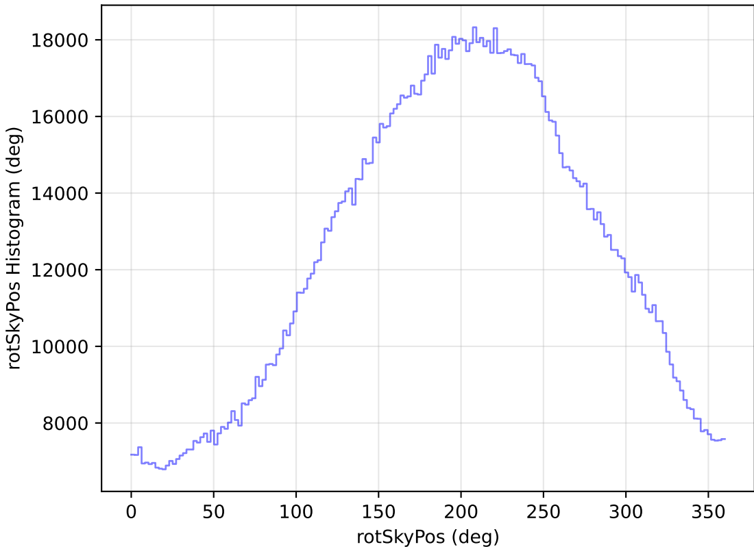
roll_pause_mjdp60_v3.4_10yrs WFD all bands: rotSkyPos Histogram
