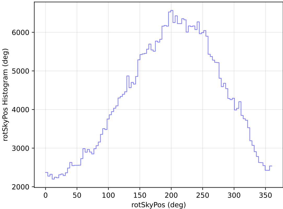
roll_pause_mjdp60_v3.4_10yrs All sky z band: rotSkyPos Histogram
