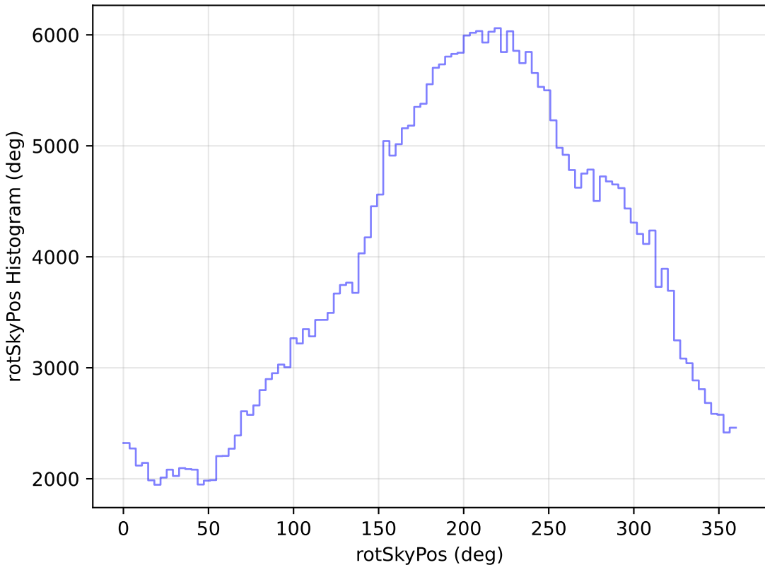
roll_pause_mjdp60_v3.4_10yrs All sky y band: rotSkyPos Histogram
