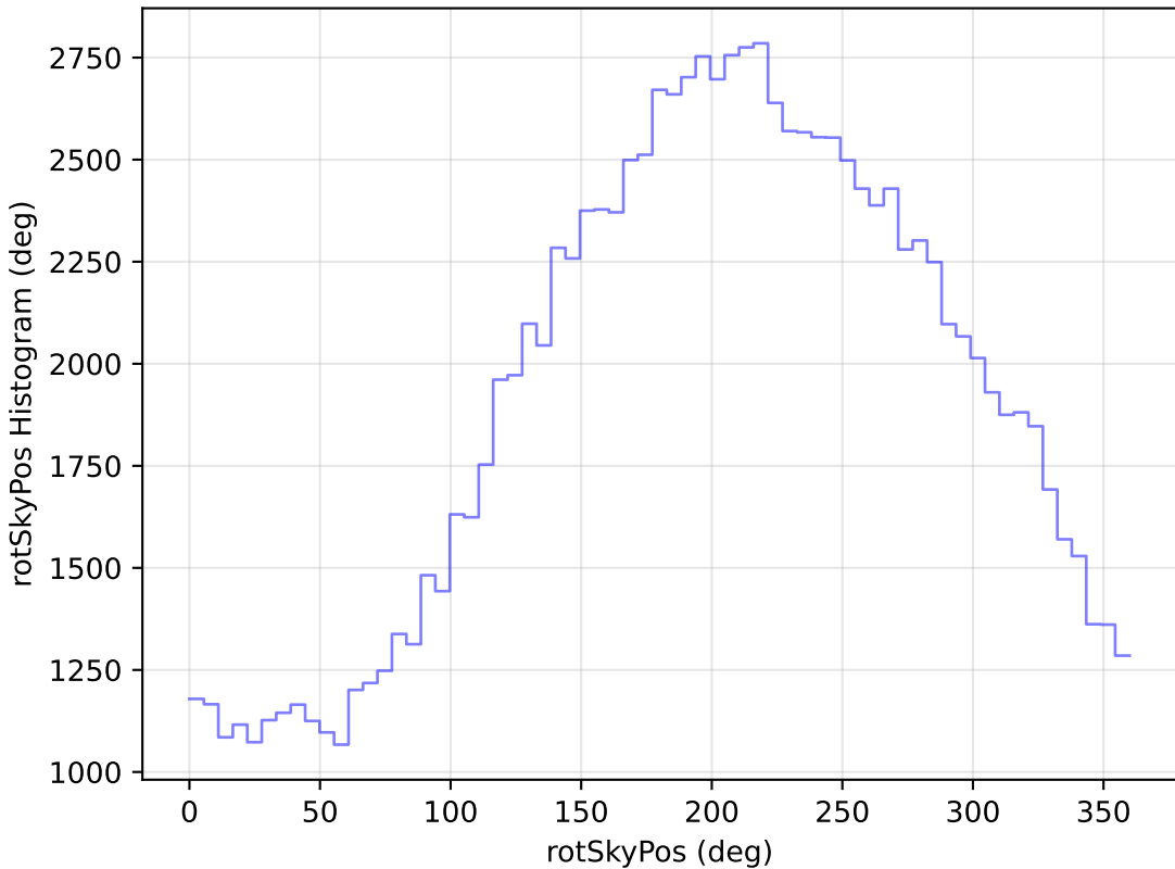
roll_pause_mjdp60_v3.4_10yrs All sky u band: rotSkyPos Histogram
