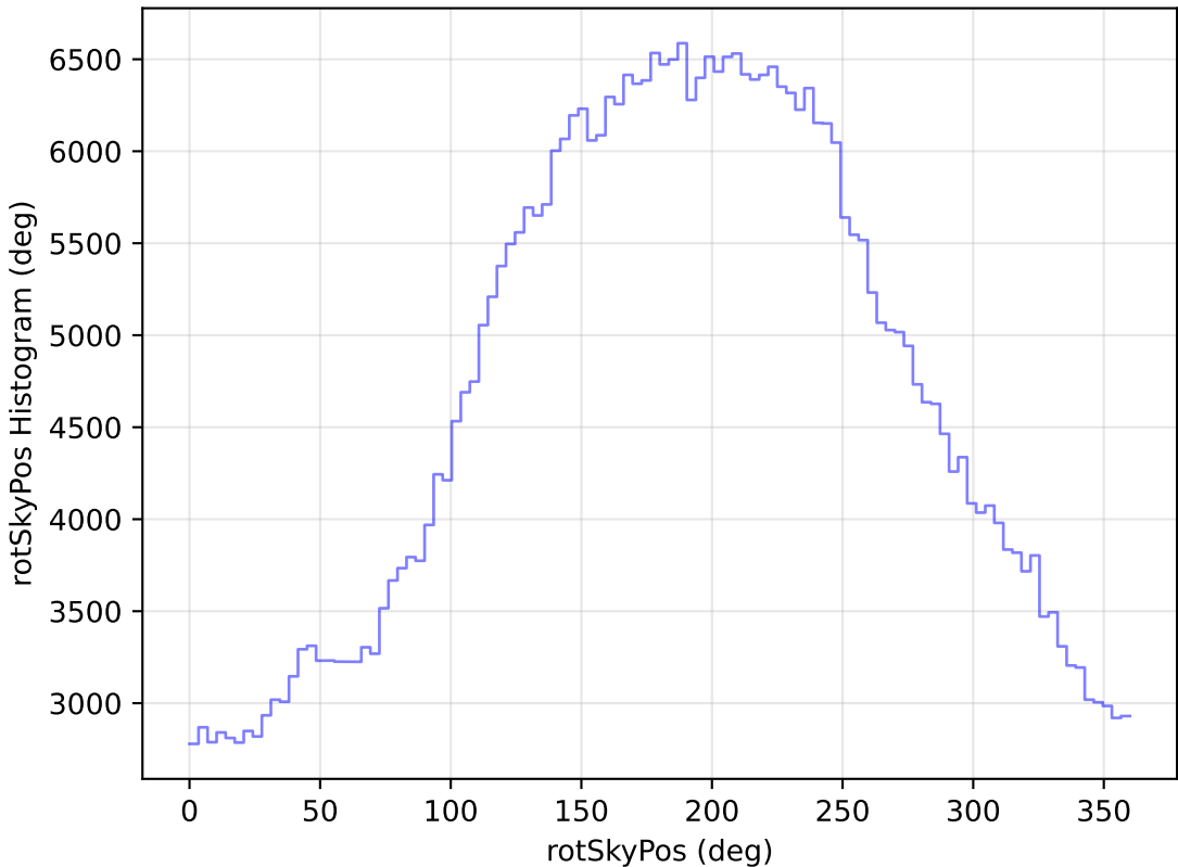
roll_pause_mjdp60_v3.4_10yrs All sky r band: rotSkyPos Histogram
