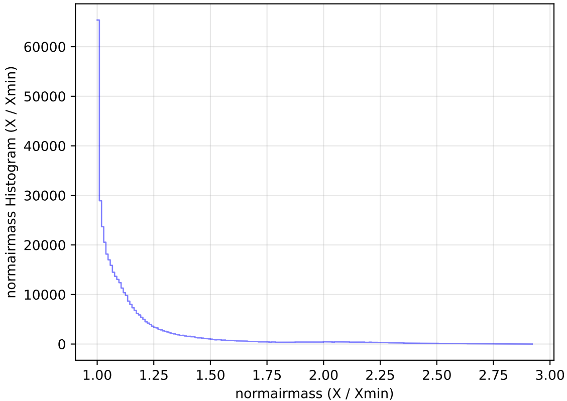
roll_pause_mjdp60_v3.4_10yrs WFD z band: normairmass Histogram
