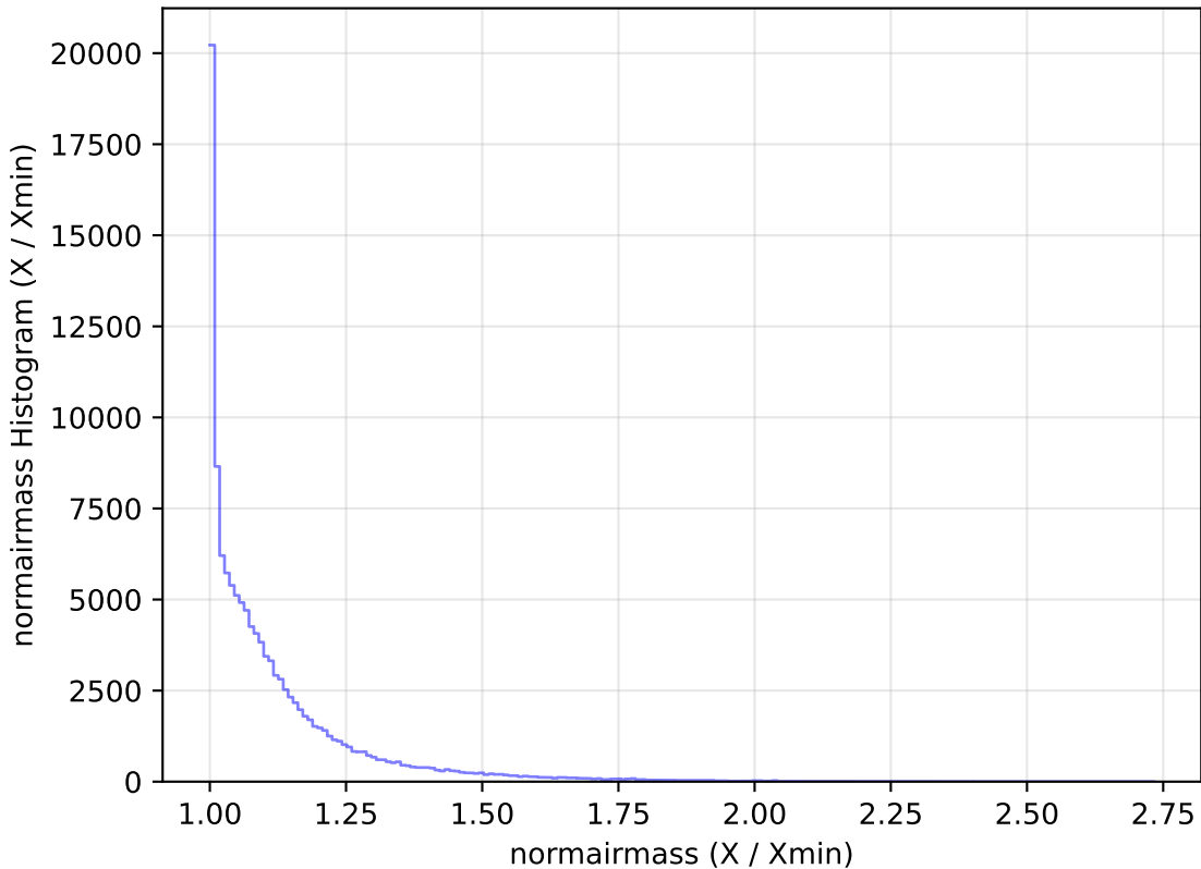
roll_pause_mjdp60_v3.4_10yrs WFD u band: normairmass Histogram
