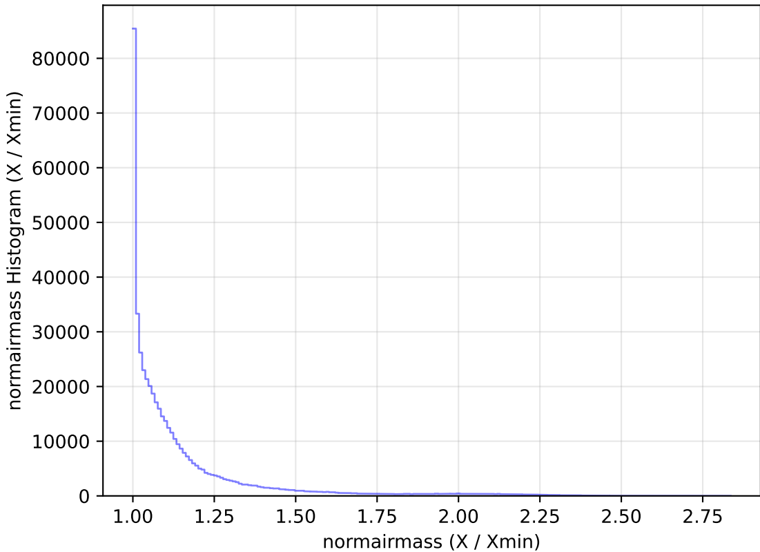
roll_pause_mjdp60_v3.4_10yrs WFD r band: normairmass Histogram
